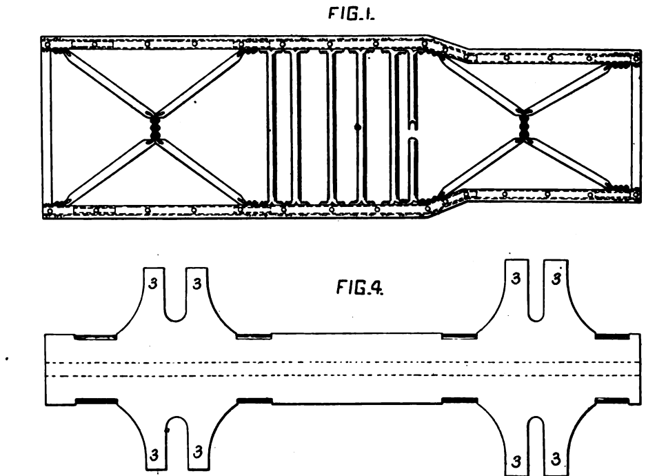
PLAN VIEW OF MARTELL PRESSED STEEL FRAME AND BLANK.
